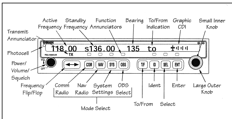
Figure 7-2. SL30 Display
